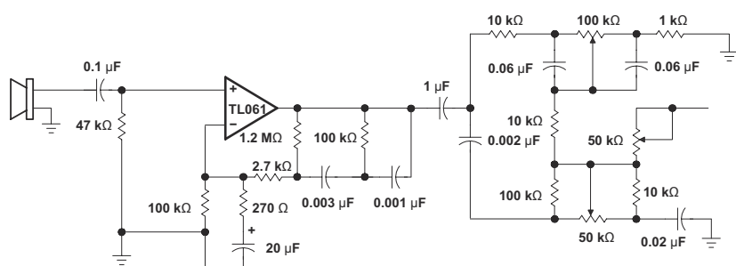
Figure 9-9. Microphone Preamplifier With Tone Control
