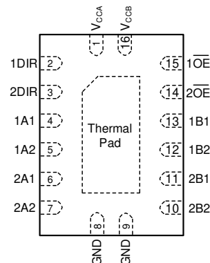
Figure 4-4. BQB/WBQB Package, 16-Pin WQFN (Transparent Top View)
