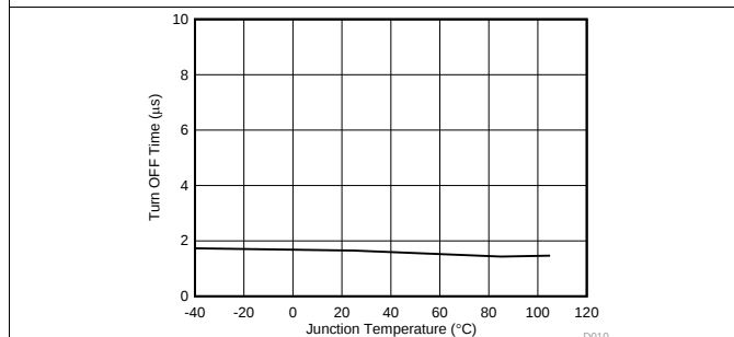
Figure 9. Turn OFF Time vs Junction Temperature
