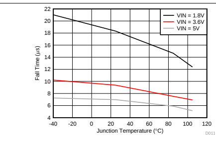
Figure 10. Fall Time vs Junction Temperature
