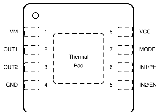
Figure 6-2. DRV8212 DSG Package 8-Pin WSON Top View
