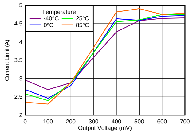
Figure 38. Foldback Current Limit vs Temperature
