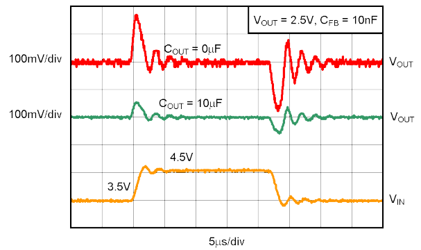
Figure 5-54. TPS73601 Line Transient, Adjustable Version
