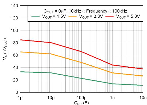
Figure 5-34. RMS Noise Voltage vs C_{NR}
