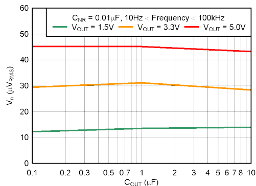
Figure 5-32. RMS Noise Voltage vs C_{OUT}
