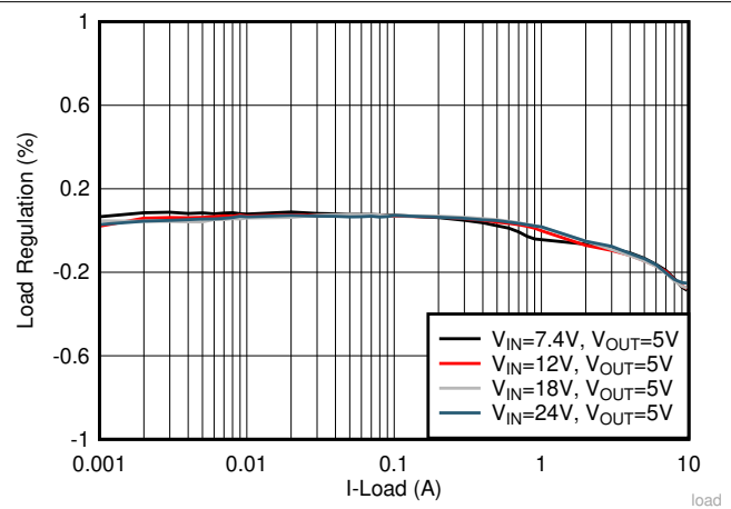
Figure 8-3. Load Regulation
