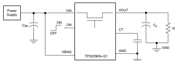
Simplified Schematic
