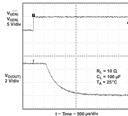
Figure 9-30. Turnoff Delay and Fall Time With 100-μF Load
