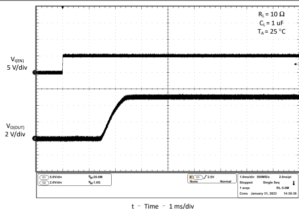
Figure 6-38. Turnon Delay and Rise Time With 1- \mu\text{F} Load
