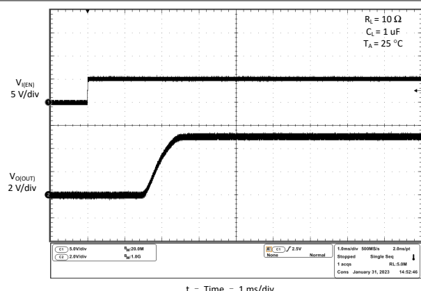
Figure 6-40. Turnon Delay and Rise Time With 100- \mu\text{F} Load
