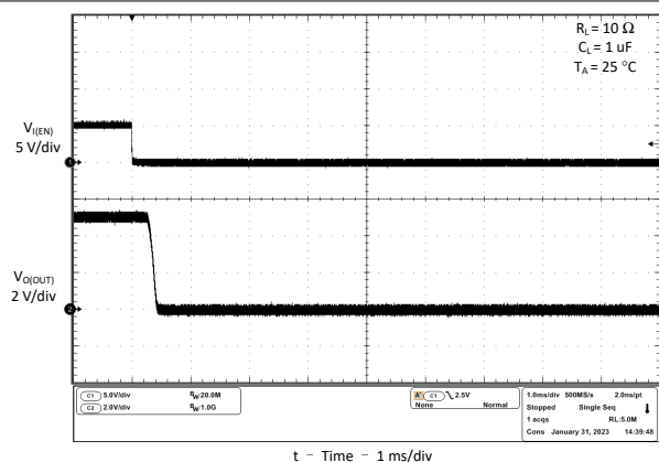
Figure 6-39. Turnoff Delay and Fall Time With 1- \mu\text{F} Load
