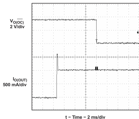
Figure 9-24. 3- \Omega Load Connected to Enabled Device
