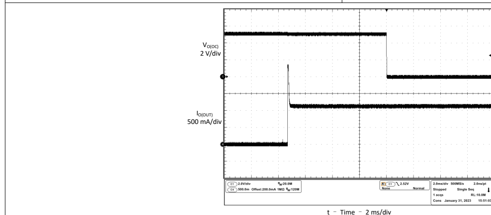
Figure 6-45. 2-Ω Load Connected to Enabled Device
