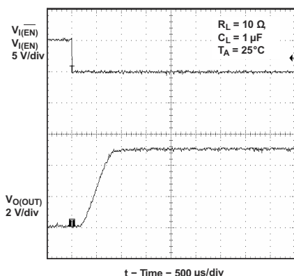
Figure 9-18. Turnon Delay and Rise Time With 1-μF Load
