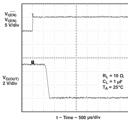
Figure 9-19. Turnoff Delay and Fall Time with 1-μF Load
