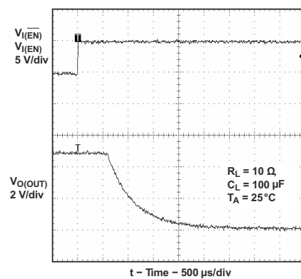
Figure 9-21. Turnoff Delay and Fall Time With 100-μF Load
