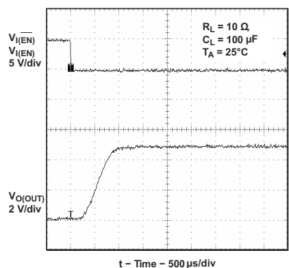
Figure 9-20. Turnon Delay and Rise Time With 100-μF Load
