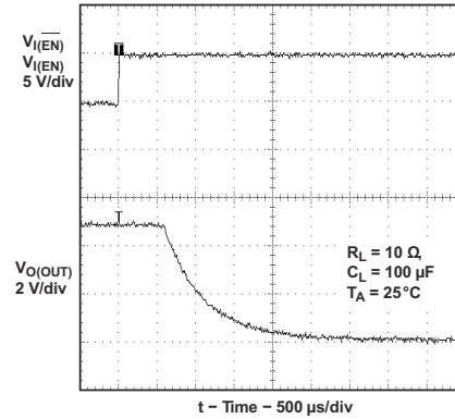
Figure 6-20. Turnoff Delay and Fall Time With 100-μF Load
