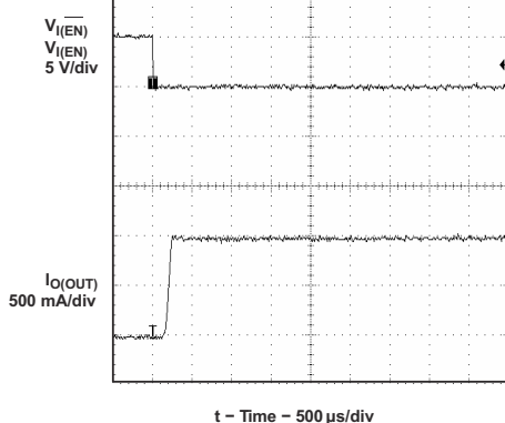
Figure 9-22. Short-Circuit Current, Device Enabled Into Short
