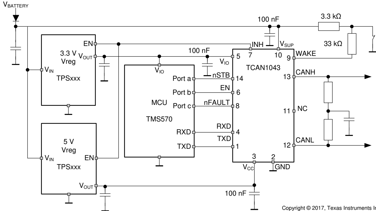
Figure 9-2. Typical CAN Bus Application Using TCAN1043xx-Q1 With 3.3 V \mu C
