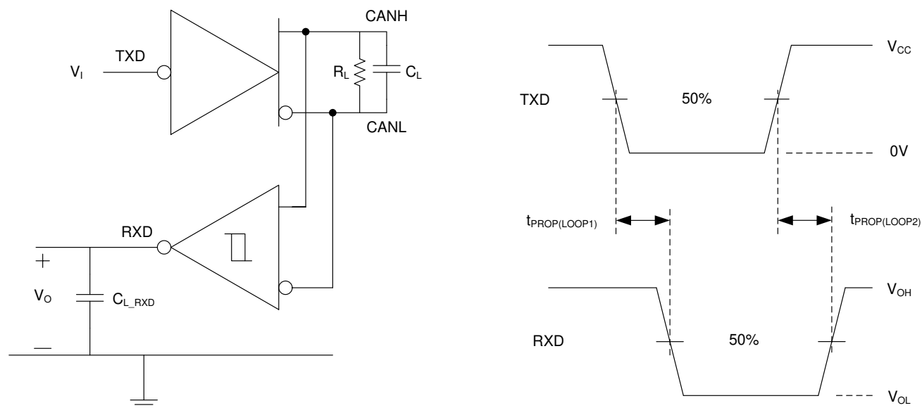
Figure 7-6. t_{\text{PROP(LOOP)}} Test Circuit and Measurement
