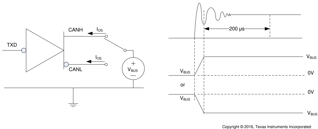
Figure 7-10. Driver Short-Circuit Current Test and Measurement
