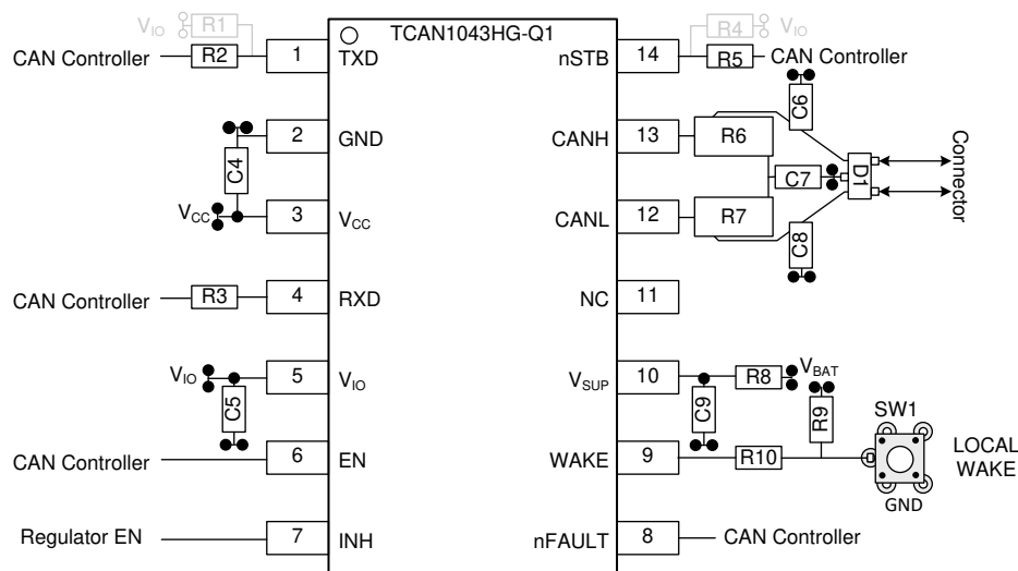
Figure 9-6. TCAN1043xx-Q1 Layout Example
