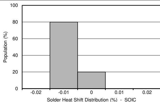
Figure 7-2. Solder Heat Shift Distribution (%), SOIC Package
