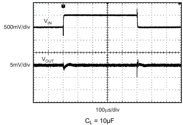
Figure 6-22. Line Transient
