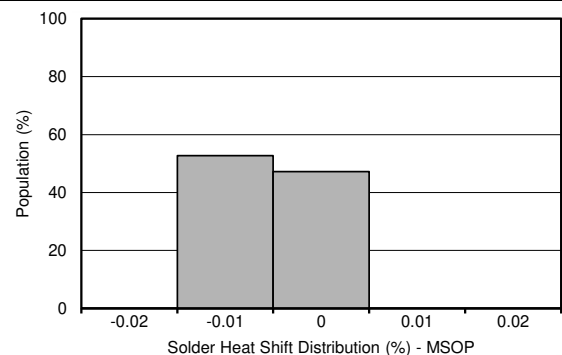
Figure 7-3. Solder Heat Shift Distribution (%), VSSOP Package
