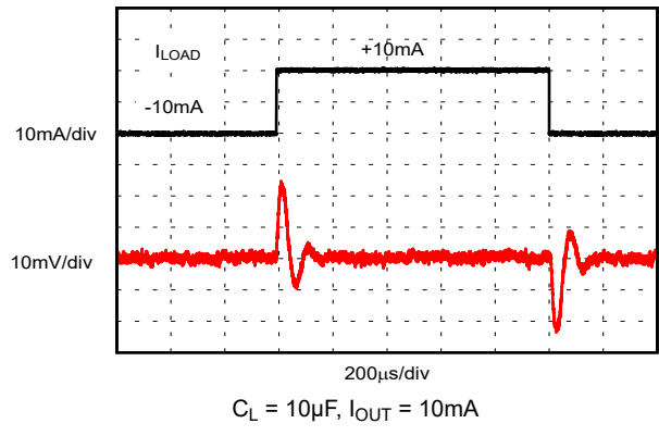
Figure 6-20. Load Transient
