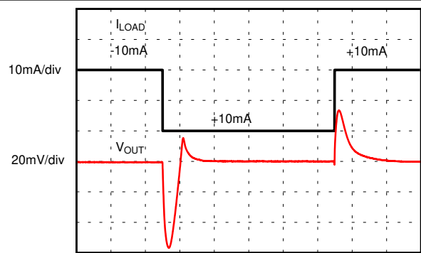
Figure 8-13. Load Transient
