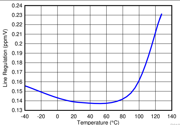
Figure 8-6. Line Regulation
