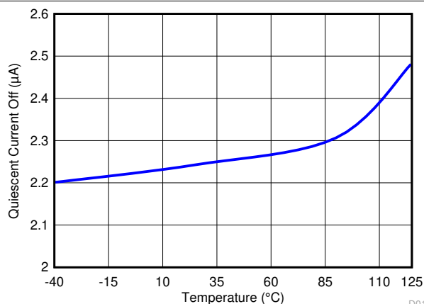
Figure 8-16. Quiescent Current Shutdown Mode
