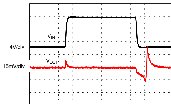
Figure 8-14. Line Transient
