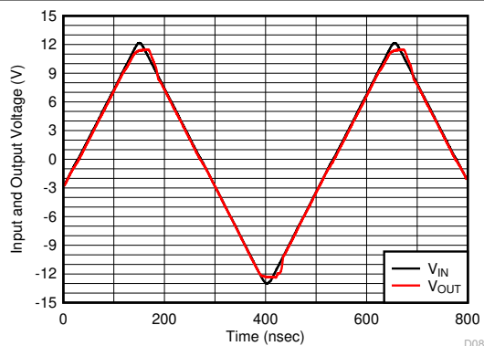
Figure 6-27. Large-Signal Transient Response
