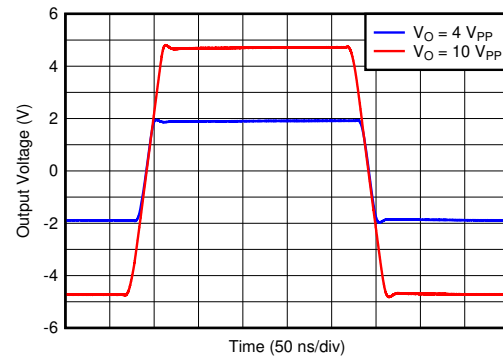
Figure 6-25. Large-Signal Transient Response
