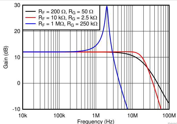
Figure 8-8. Closed-Loop Gain vs. Frequency for Circuit of Figure 8-5
