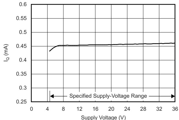
Figure 5-18. Quiescent Current vs Supply Voltage
