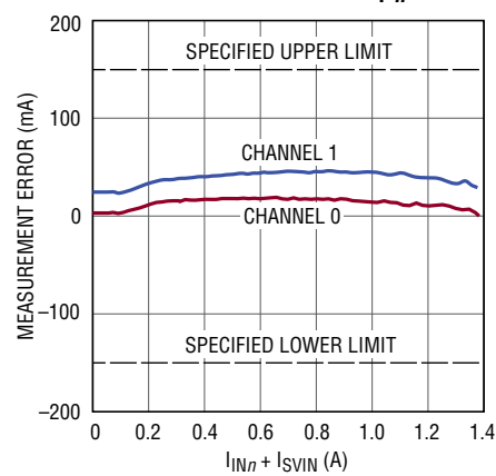
MFR_READ_IIN n (Input Current Readback) Error vs (I_{\text{VIN}n} + I_{\text{SVIN}}) , \text{MFR\_PWM\_MODE}_n[0]=1_b , I_{\text{OUT}n} Swept from 0A to 13A, One Channel at a Time, \text{RUN}_{1-n} = 0\text{V}
