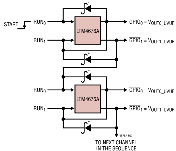
Voltage Based Sequencing by Cascading \overline{\text{GPIO}}_n Pins Into \text{RUN}_n Pins (IFR_GPIO_PROPAGATE = XXX1X00XX0XXXX b and MFR_GPIO_RESPONSE = 0x00)
