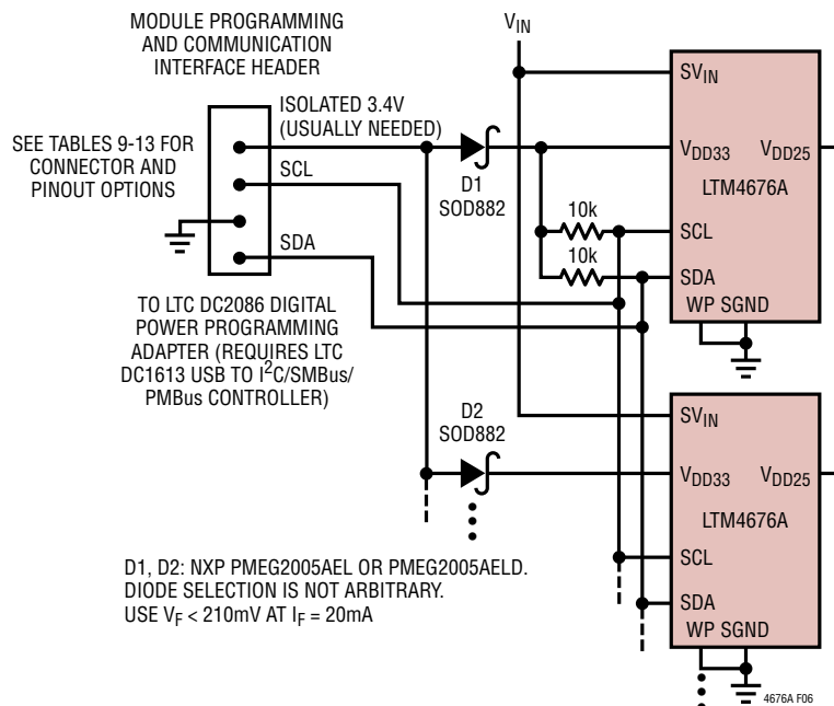
Figure 6. Circuit Suitable for Programming EEPROM/NVM of LTM4676A and Other ADI PSM Modules/ICs in Vast Systems, Even When V_{IN} Power is Absent, T_A > 20^{\circ}\text{C} and T_J < 85^{\circ}\text{C}
