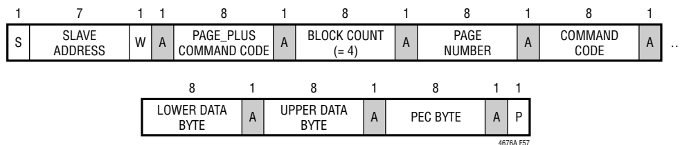
Figure 63. Example of PAGE_PLUS_WRITE
