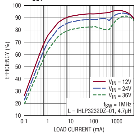
LT8637 Low Load Efficiency at 5V OUT
