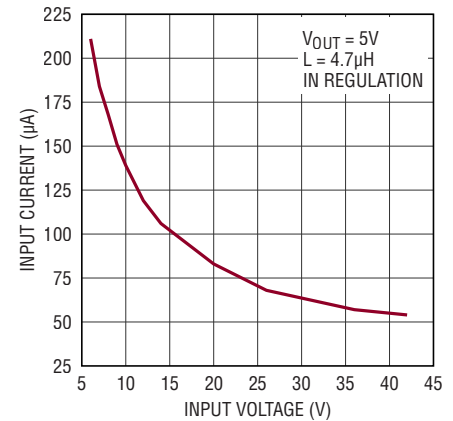
LT8637 No-Load Supply Current
