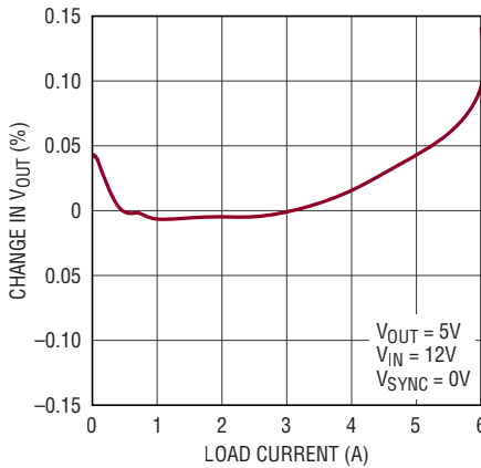
LT8636 Load Regulation
