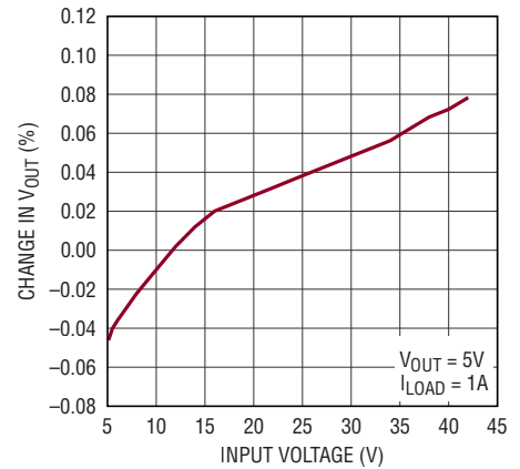
LT8636 Line Regulation
