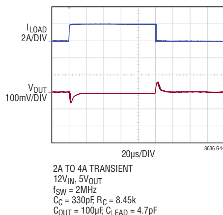
LT8637 Transient Response; External Compensation
