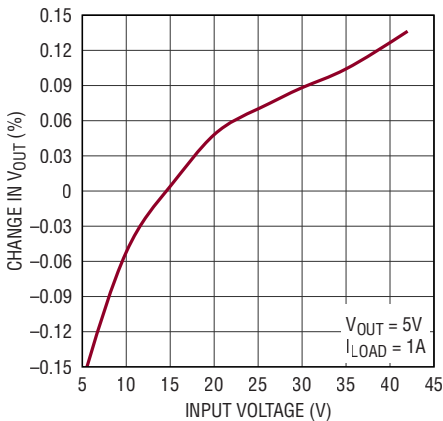
LT8637 Line Regulation
