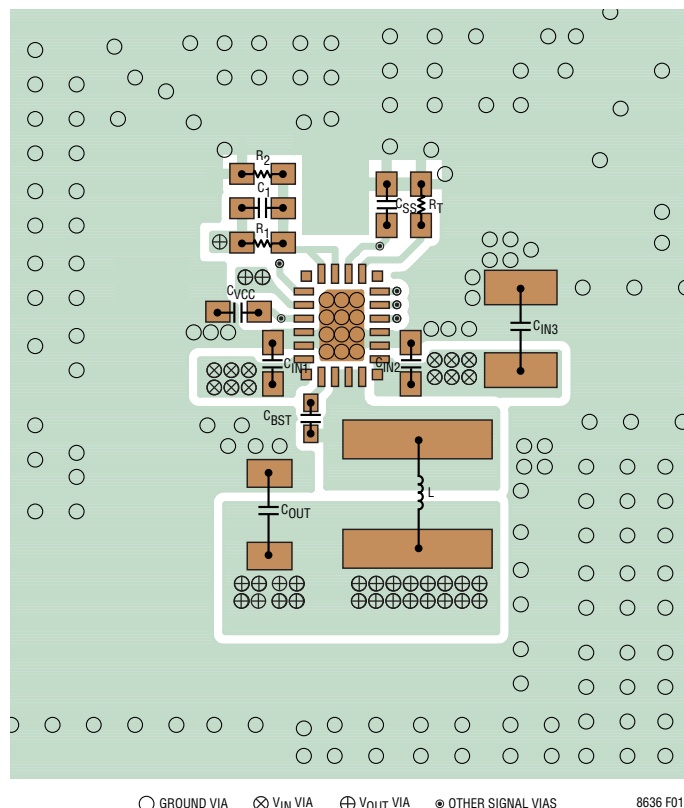
(a) LT8636
