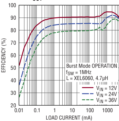
LT8636 Low Load Efficiency at 3.3V OUT
