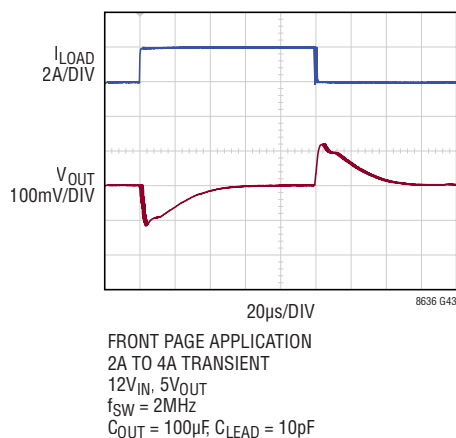
LT8636 Transient Response; Internal Compensation
