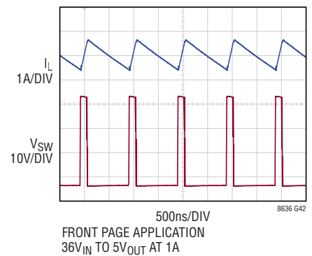
Switching Waveforms
