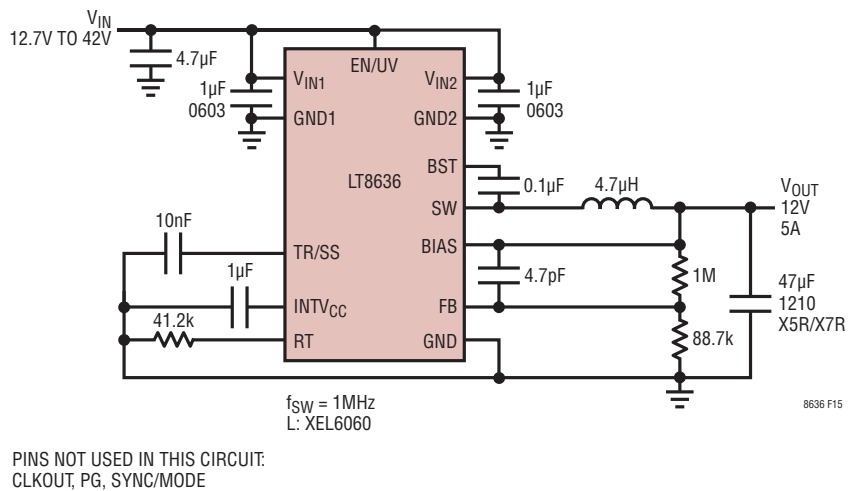
Figure 15. 12V, 5A Step-Down Converter
