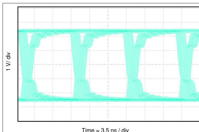
Figure 9-3. ISO7720 Eye Diagram at 100 Mbps PRBS, 5-V Supplies and 25°C
