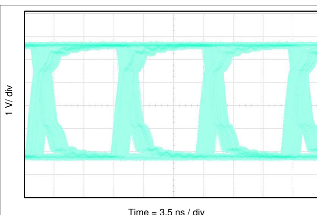
Figure 9-4. ISO7721 Eye Diagram at 100 Mbps PRBS, 5-V Supplies and 25°C
