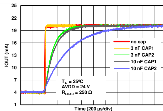
Figure 8-7. IOUT vs Time for Different Capacitor Values on CAP1 and CAP2
