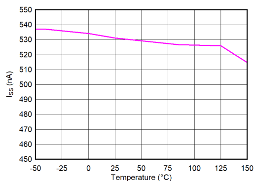
Figure 5-30. Soft-Start Charging Current ( I_{SS} ) vs Temperature ( T_J )
