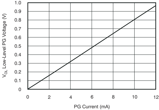
Figure 5-31. Low-Level PG Voltage vs PG Current
