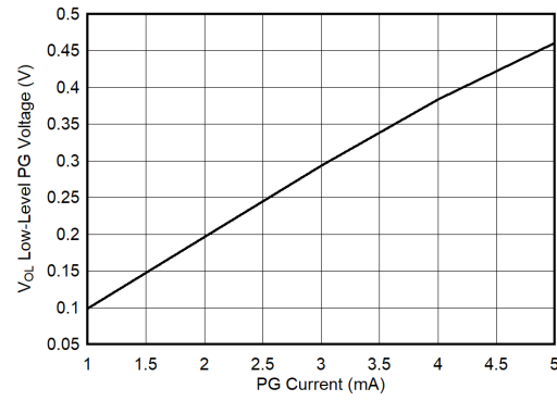
Figure 5-32. Low-Level PG Voltage vs Current
