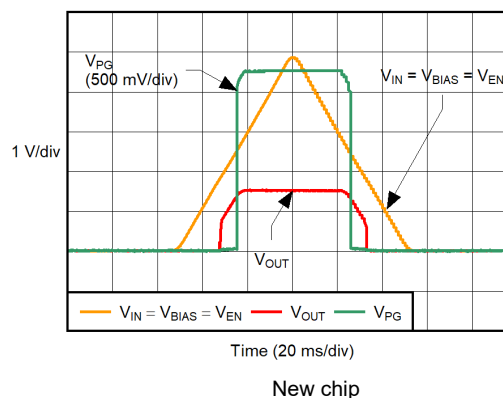
Figure 5-42. Power-Up, Power-Down
