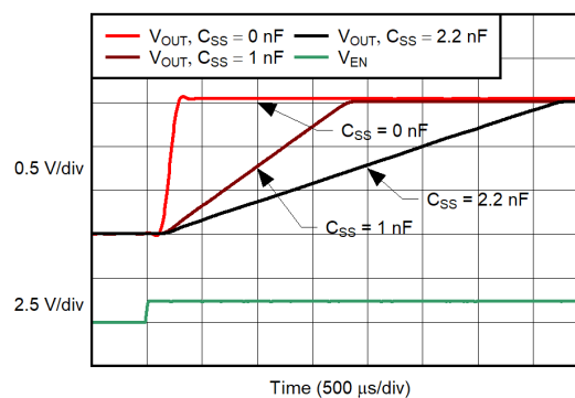
Figure 5-40. Turn-On Response
