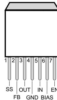
Figure 4-2. KTW Package 7-Pin DDPAK Top View
