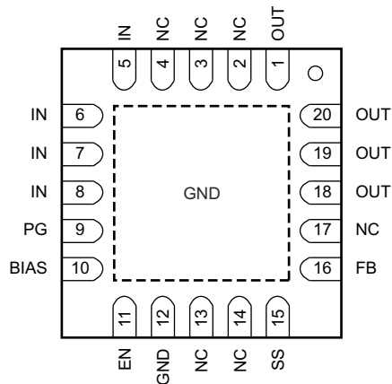
Figure 4-1. RGW, RGR Package 5mm × 5mm and 3.5mm × 3.5mm, 20-Pin VQFN Top View
