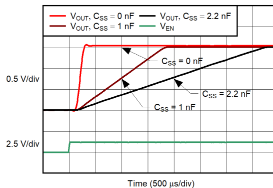
Turn-On Response
