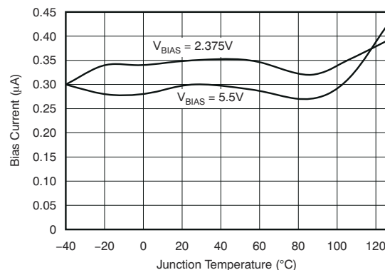
Figure 5-28. I_{BIAS} Shutdown vs Temperature
