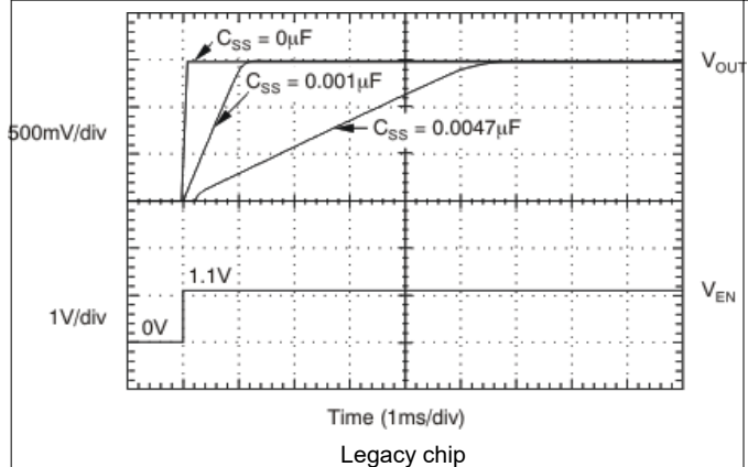
Figure 5-39. Turn-On Response
