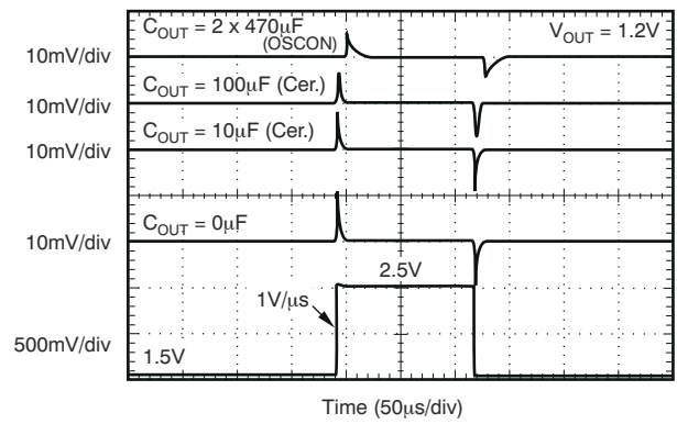
Figure 7-5. V_{IN} Line Transient (3A)
