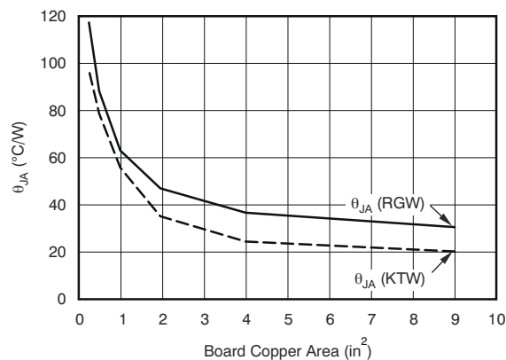
Figure 7-14. \theta_{JA} versus Board Size
