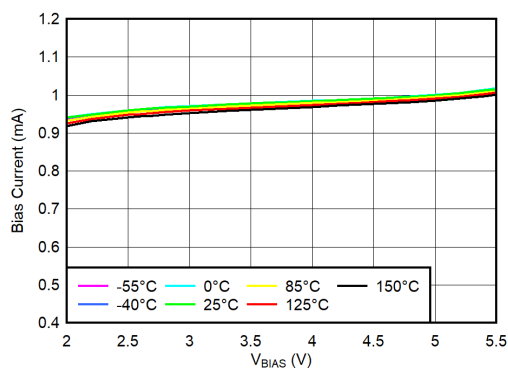
Figure 5-27. BIAS Pin Current vs V_{BIAS} and Temperature ( T_J )
