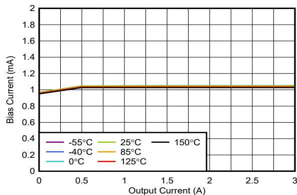
Figure 5-25. BIAS Pin Current vs Output Current and Temperature ( T_J )
