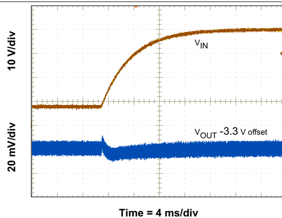
Figure 35. Line Transient (8 V to 40 V)
