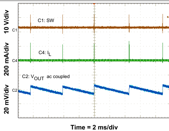
Figure 40. Output Ripple PSM
