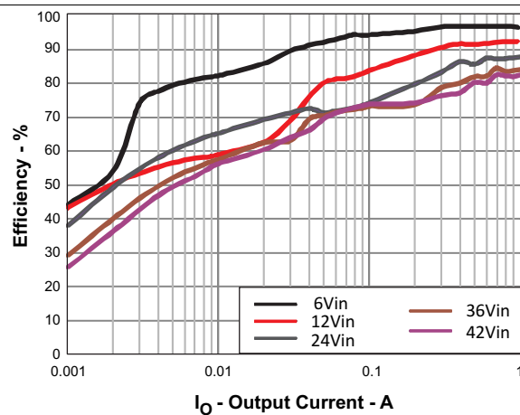
Figure 47. Light-Load Efficiency
