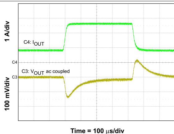
Figure 34. Load Transient
