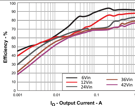
Figure 45. Light-Load Efficiency
