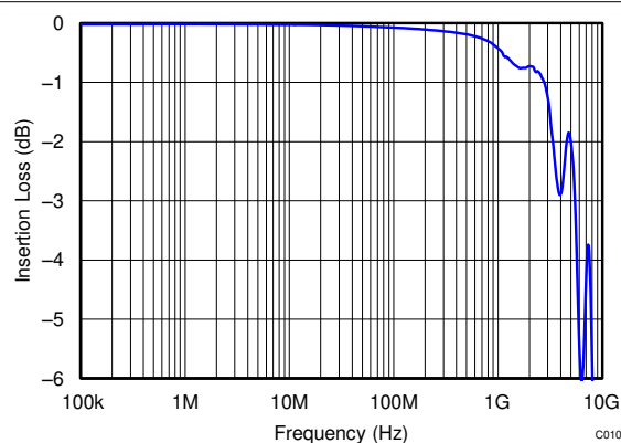
Figure 5-10. TPD6E05U06 Insertion Loss
