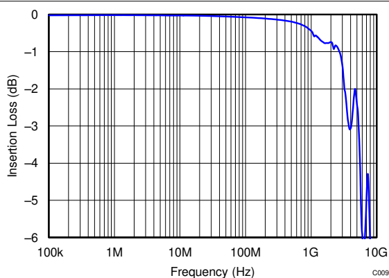
Figure 5-9. TPD4E05U06 Insertion Loss
