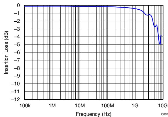
Figure 5-8. TPD1E05U06 Insertion Loss
