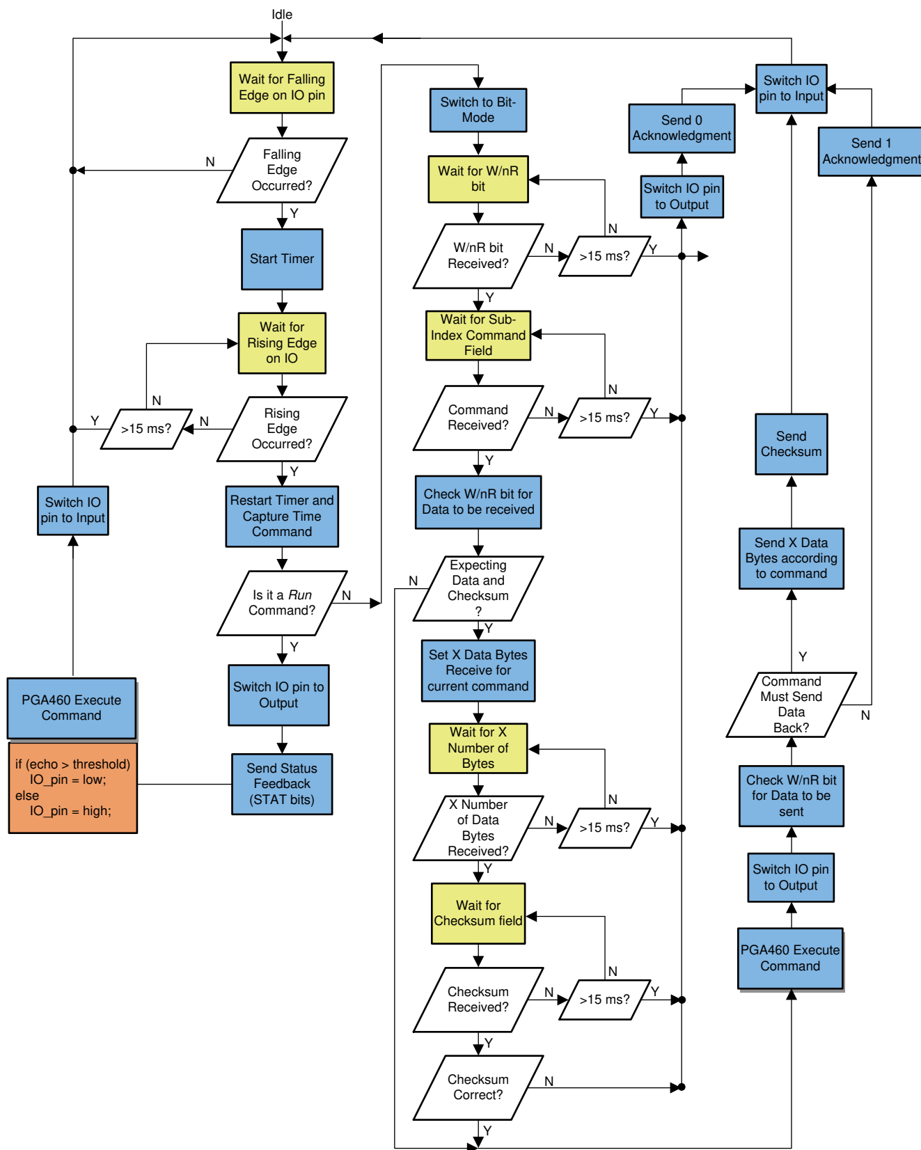
Figure 7-42. Time-Command Interface Communication Flow Chart
