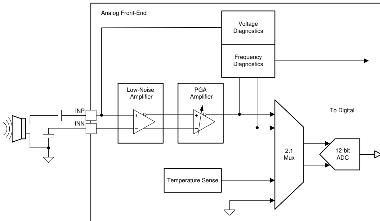
Figure 7-3. Analog Front-End
