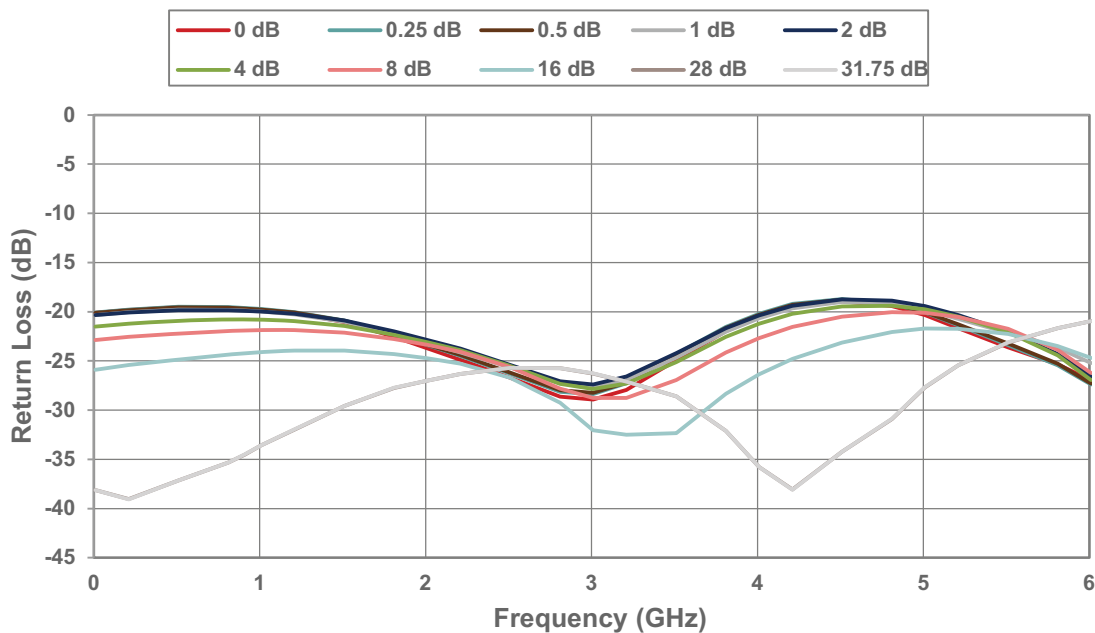
Figure 7 ■ Input Return Loss vs Attenuation Setting
