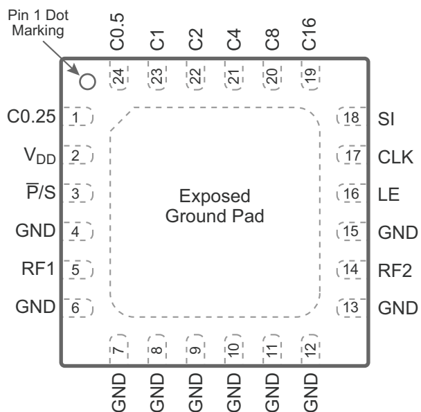
Figure 35 ■ Pin Configuration (Top View)
