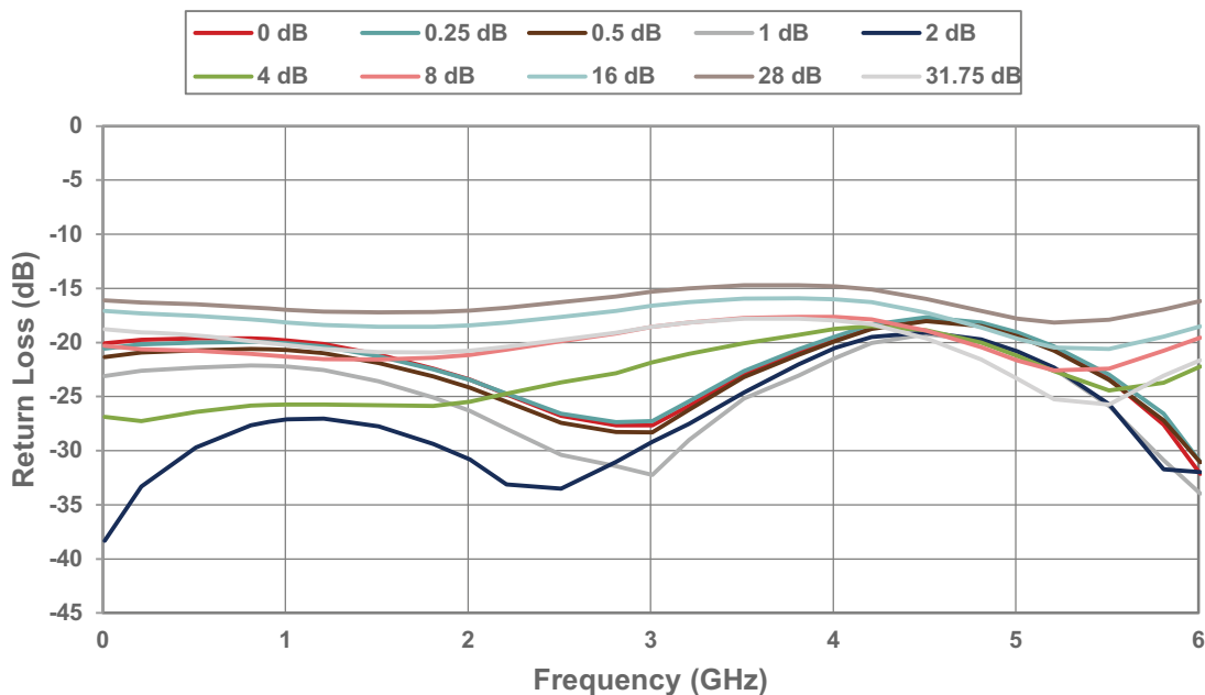
Figure 8 ■ Output Return Loss vs Attenuation Setting
