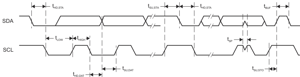
Figure 8-18. I 2 C Mode Timing
