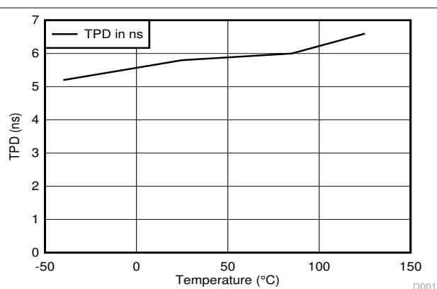
Figure 6-2. Temperature 1.8 V, 15 pF Load
