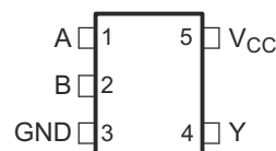
Figure 5-2. DRL Package SOT 5-pin (Top View)
