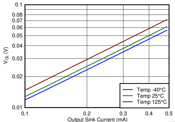
V_{CC} = 1.8\text{V}
