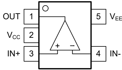
Figure 4-2. TLV70x1L "LMC72x5 type" Pinout with reversed supplies DBV Package, SOT-23-5 Top View
