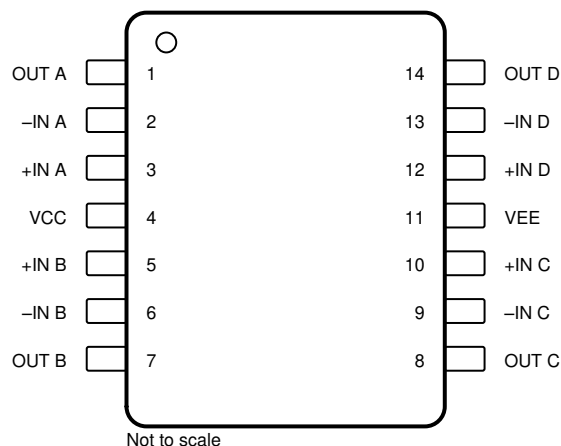
Figure 4-7. TLV7034/44 PW Packages 14-Pin TSSOP Top View
