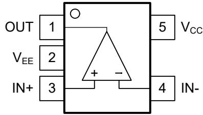
Figure 4-1. TLV70x1 Standard "North West" Pinout DBV, DCK, Packages, SOT-23-5, SC-70-5 Top View
