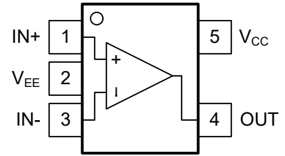
Figure 4-3. TLV70x1S Standard "South East" Pinout DBV, DCK Packages, SOT-23-5, SC-70-5 Top View
