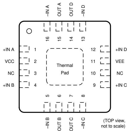
Figure 4-8. TLV7034/44 RTE Package 16-Pin WQFN With Exposed Thermal Pad Top View
