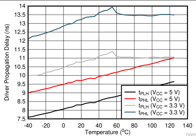
Figure 6-8. THVD2450 Driver Propagation Delay vs Temperature
