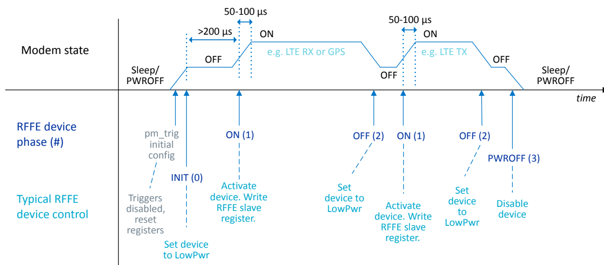
Figure 111: MIPI RFFE interface timing
