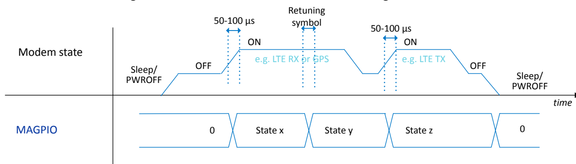
Figure 112: MAGPIO interface timing
