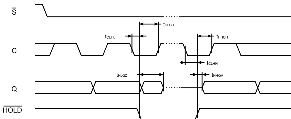
Figure 21. Hold timing
